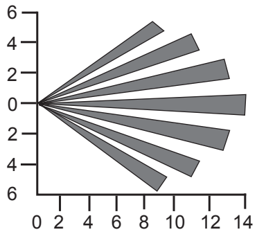
BEAM PATTERN SET TO MINIMUM RANGE. MASKING TOP SECTION LENS WILL REDUCE RANGE TO 6 METRES
