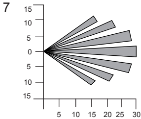
Beam Pattern set to maximum range - Masking top section of lens will reduce to 20 metres
