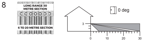
Beam Pattern set to maximum range - Masking top section of lens will reduce to 20 metres
