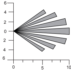
Beam Pattern set to minimum range - Masking top section of lens will reduce to 6 metres
