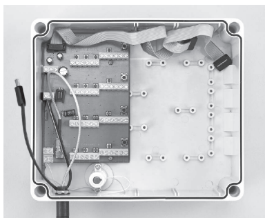
fig 1 STANDARD RECEIVER UNIT WITH PRE-INSTALLED 4 CHANNEL MODULE
